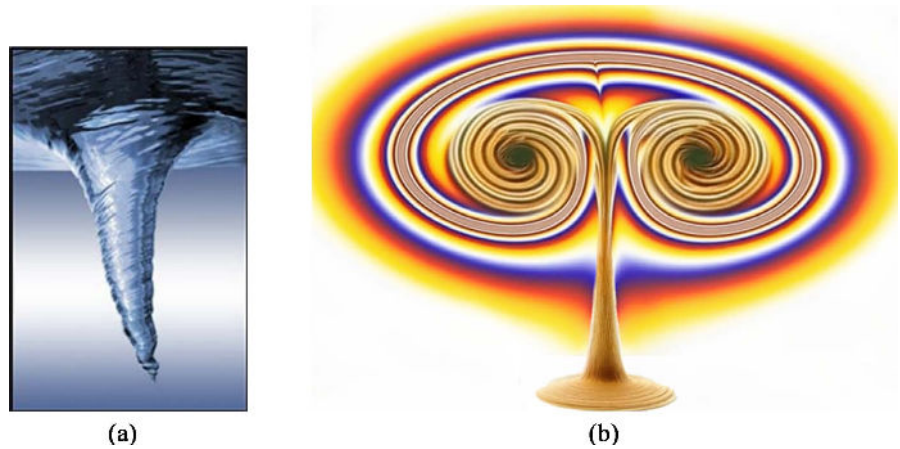
Figure 2. (a) Whirlpool Vortex Tapering, the radius decreases as angular velocity and energy density increase toward the core. (b) The image illustrates the vortex-based geometry of the proton, with two up quark vortices forming the upper symmetrical spirals and the down quark forming the central tapered stem. The relative size and shape reflect the spatial and energetic proportions between quarks, supporting the mushroom-like structure of the proton in the Quark Vortex Model.
